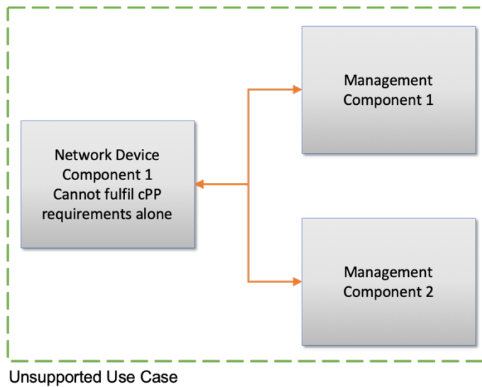
Figure 11: Unsupported use case with Multiple Management Components
