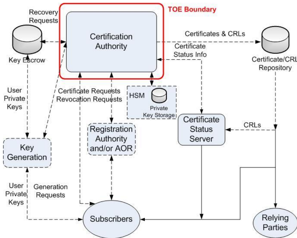
Figure 1 - TOE Boundary in Example PKI Architecture
